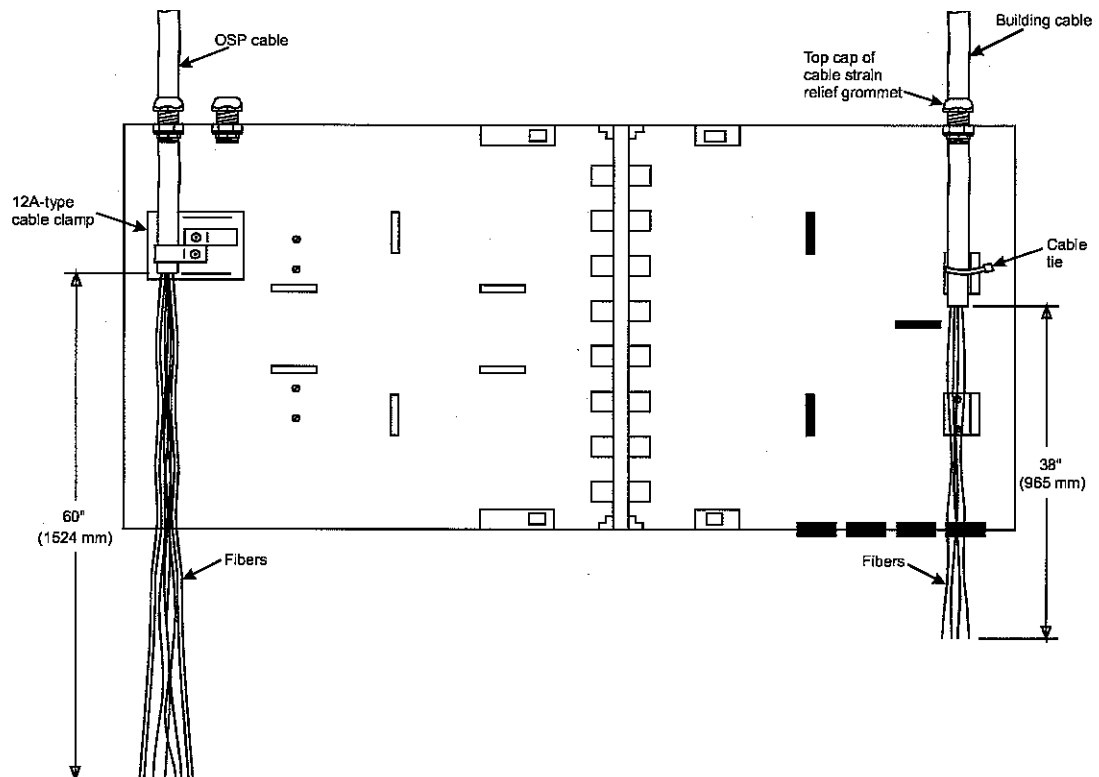
Figure 11—Interconnection Cabling
